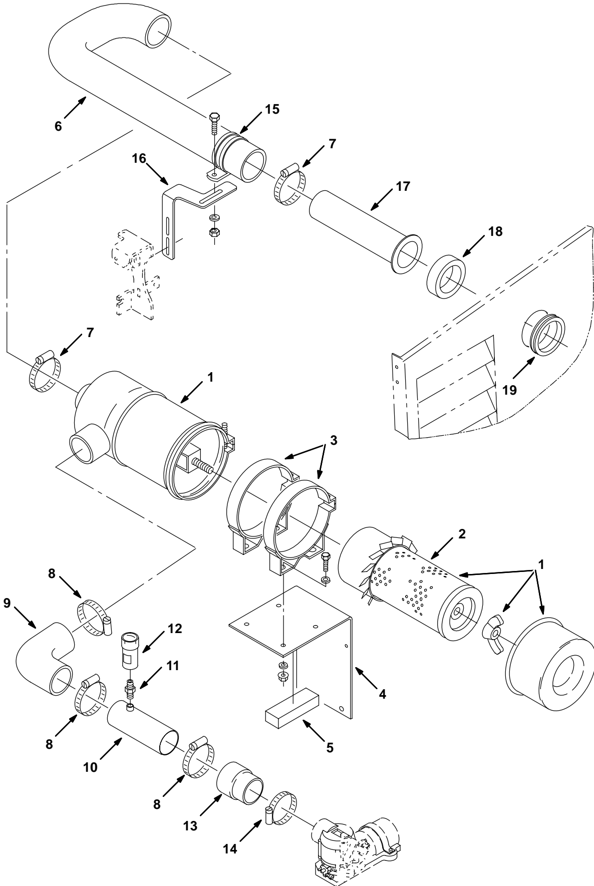
Fig. 45 – Air Cleaner Group, LPG
