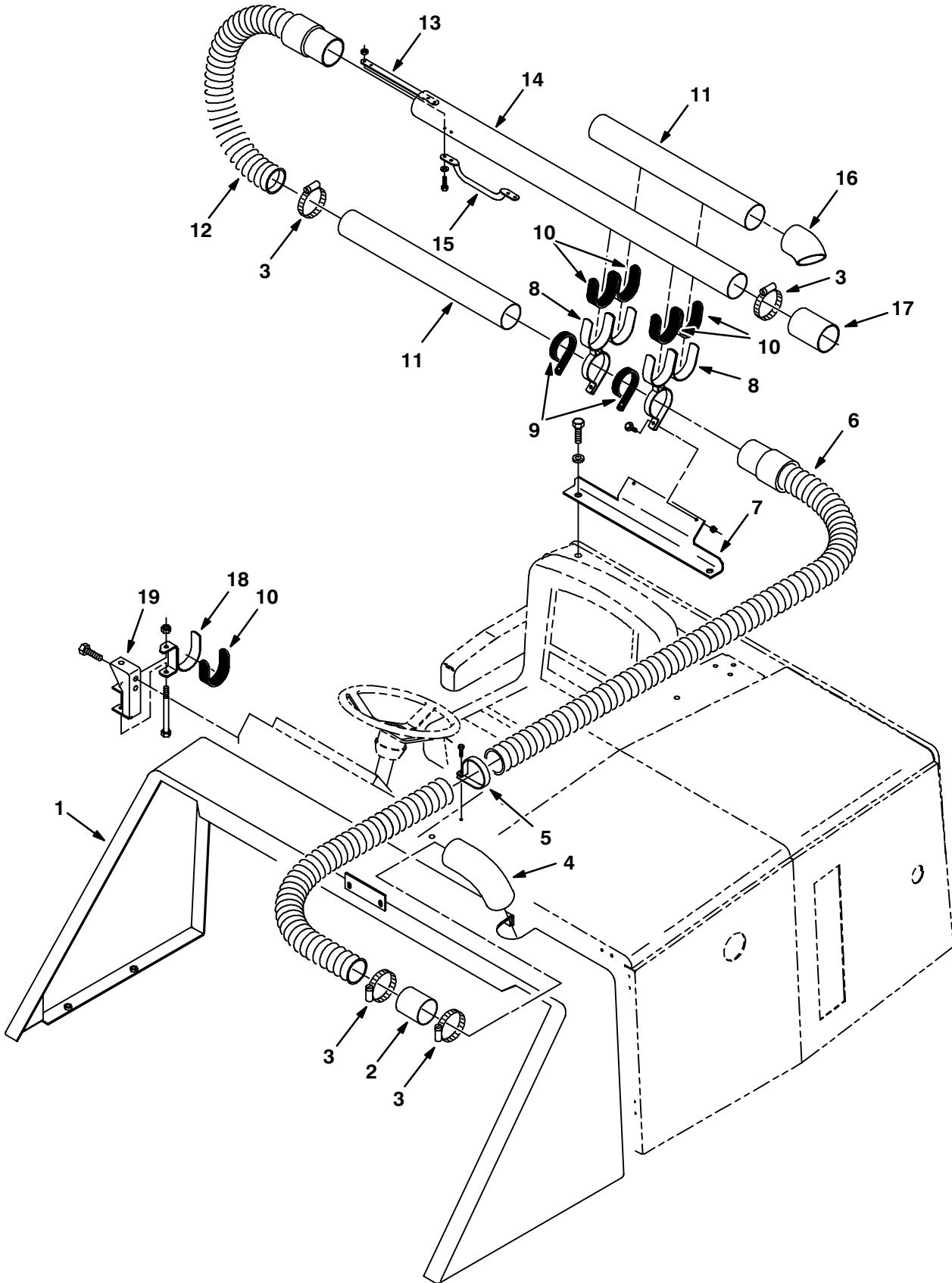
Fig. 12 – Blower Group
