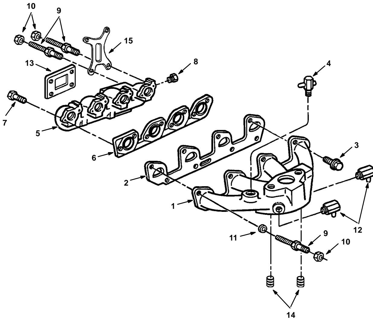
Fig. 8 – Manifolds Group
