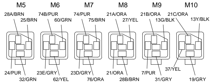
VIEW M-M
