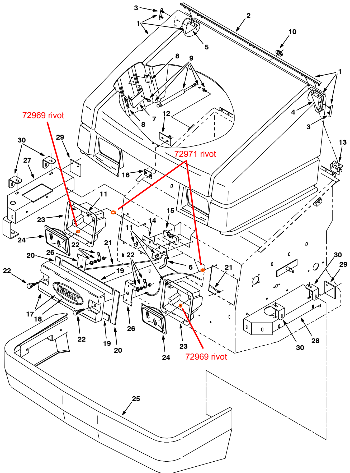
Fig. 33 - Hopper Hood and Bumper Group
