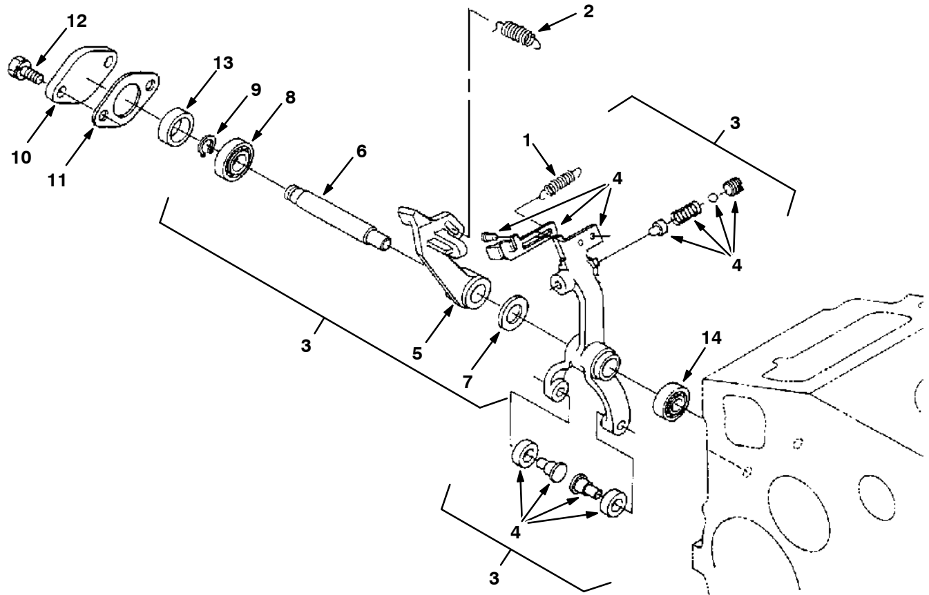
Fig. 23 - Governor Group
