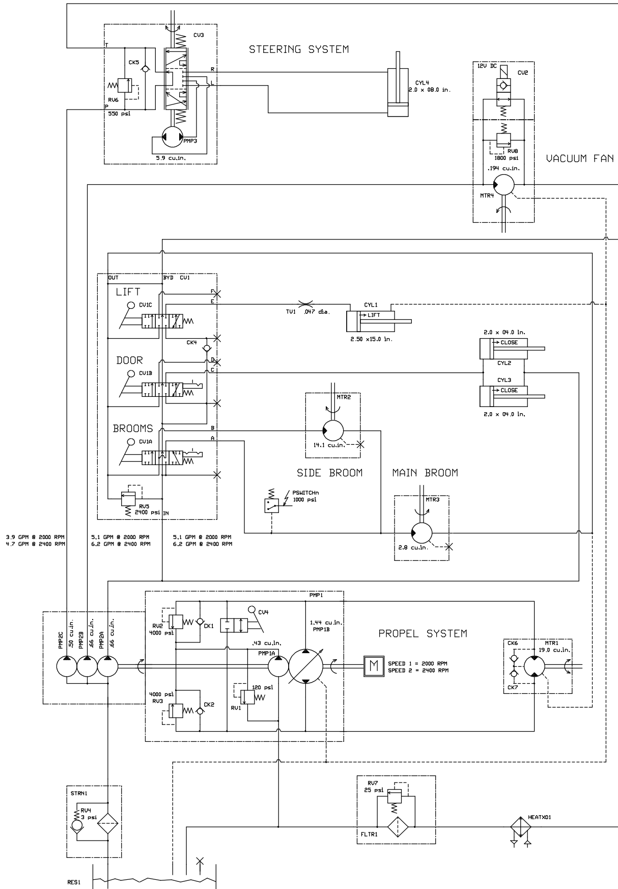
Fig. 43 - Hydraulic Schematic
