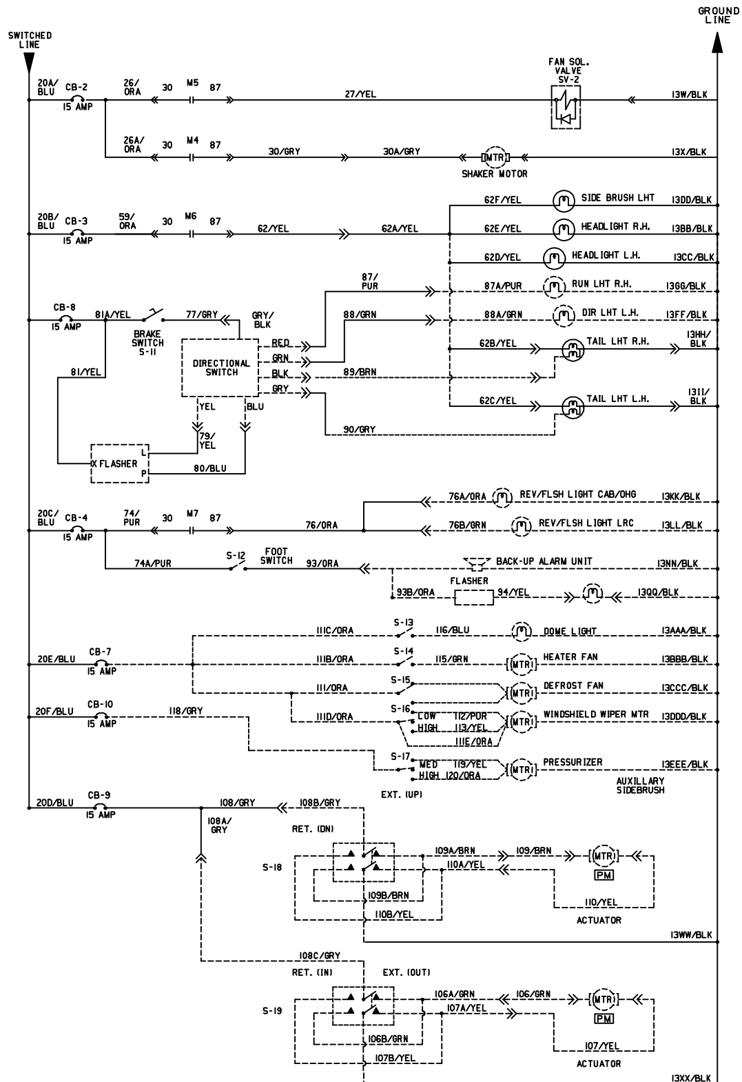
Fig. 52 - Electrical Schematic
