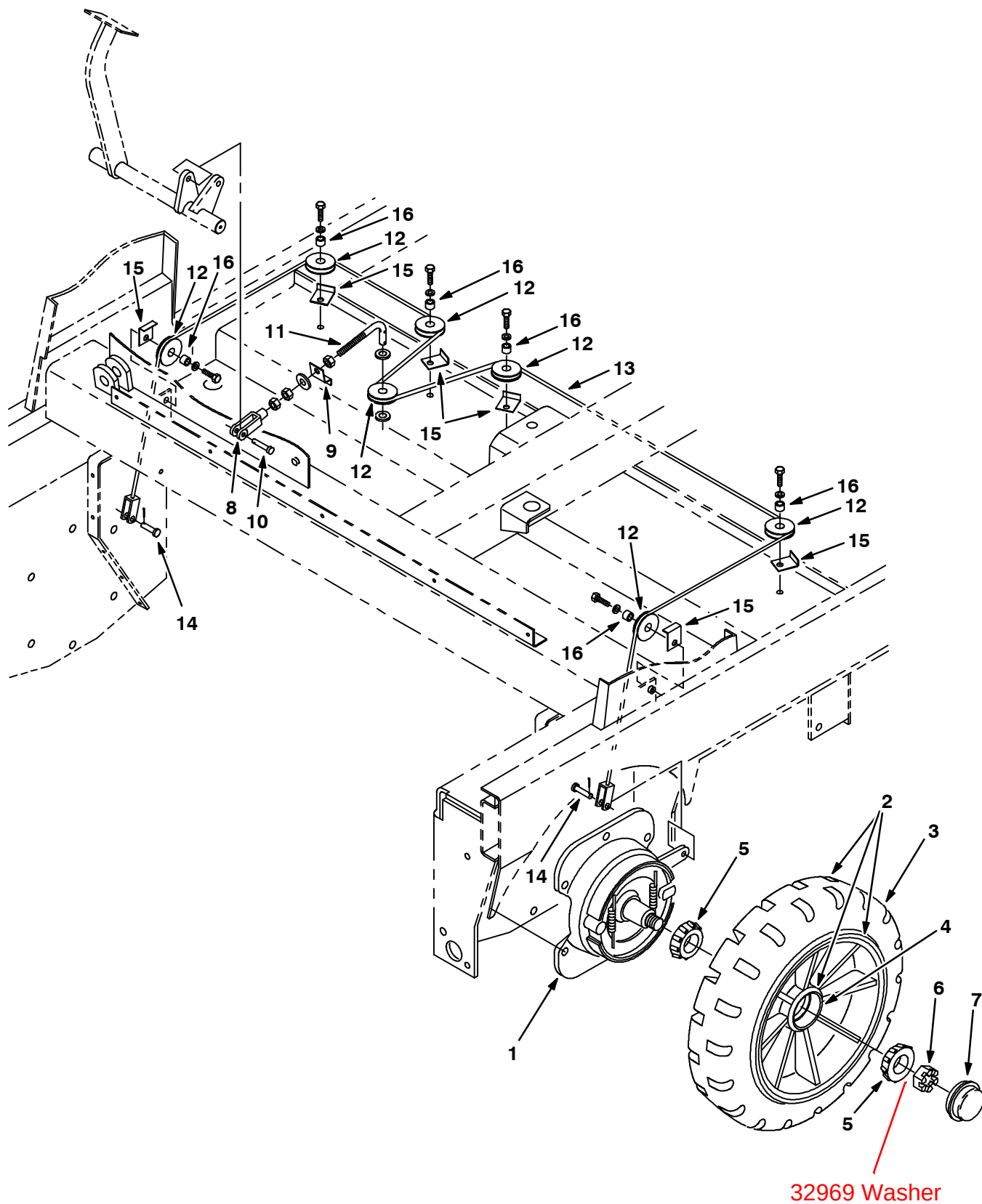
Fig. 27 - Front Wheel and Brakes Group
