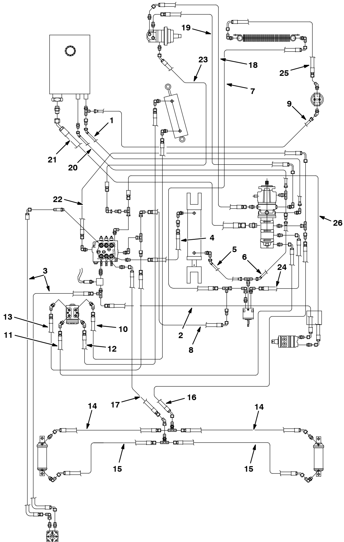
Fig. 45 - Hydraulic Hose Group
