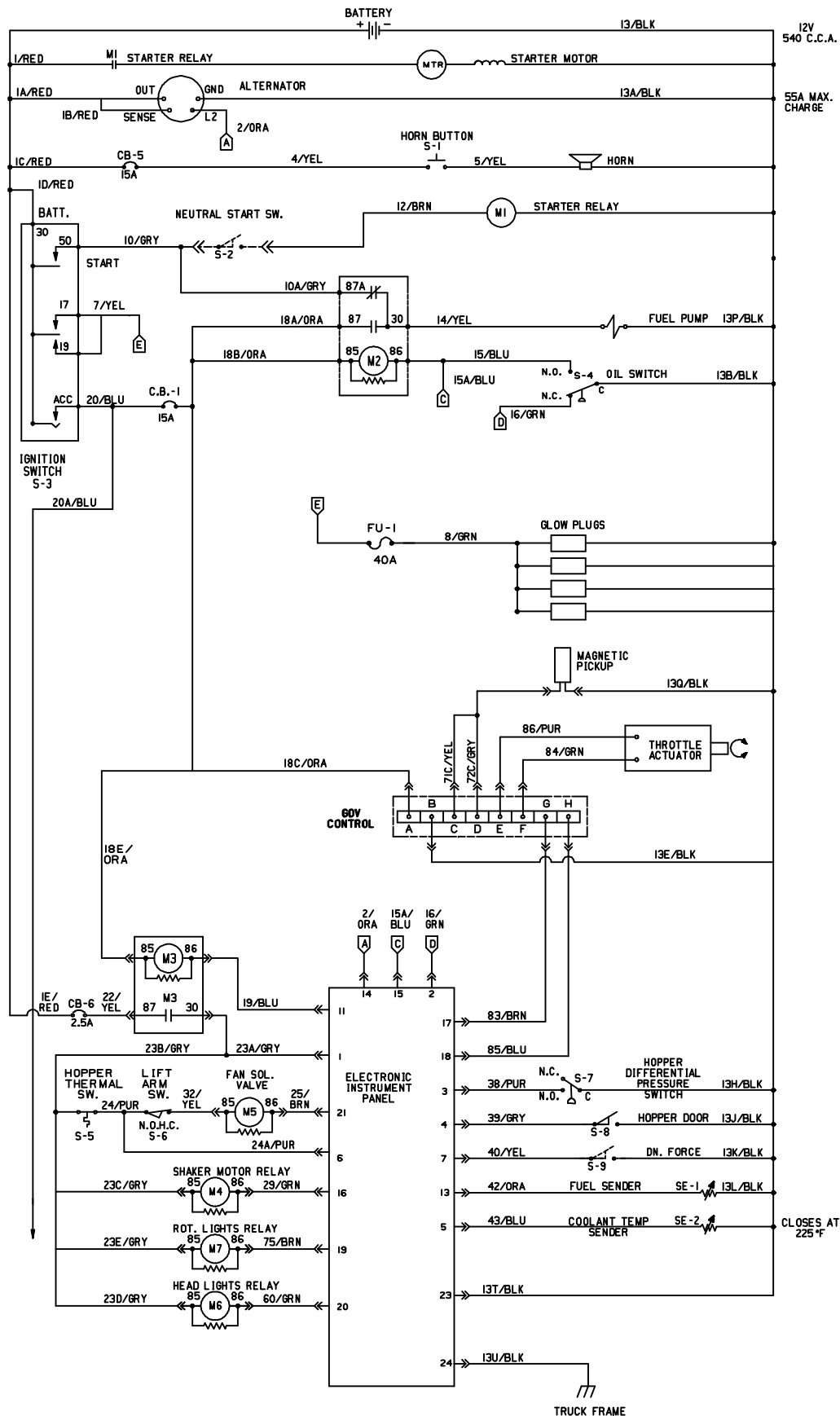
Fig. 52 - Electrical Schematic
