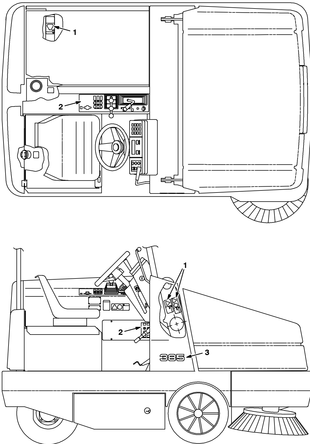
Fig. 54 - Label Group
