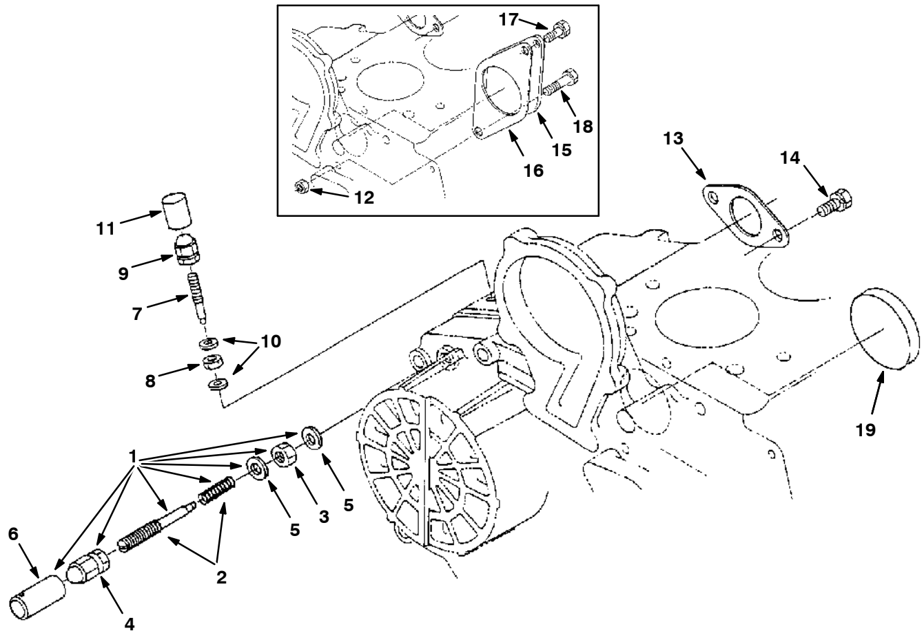
Fig. 21 - Idling Group
