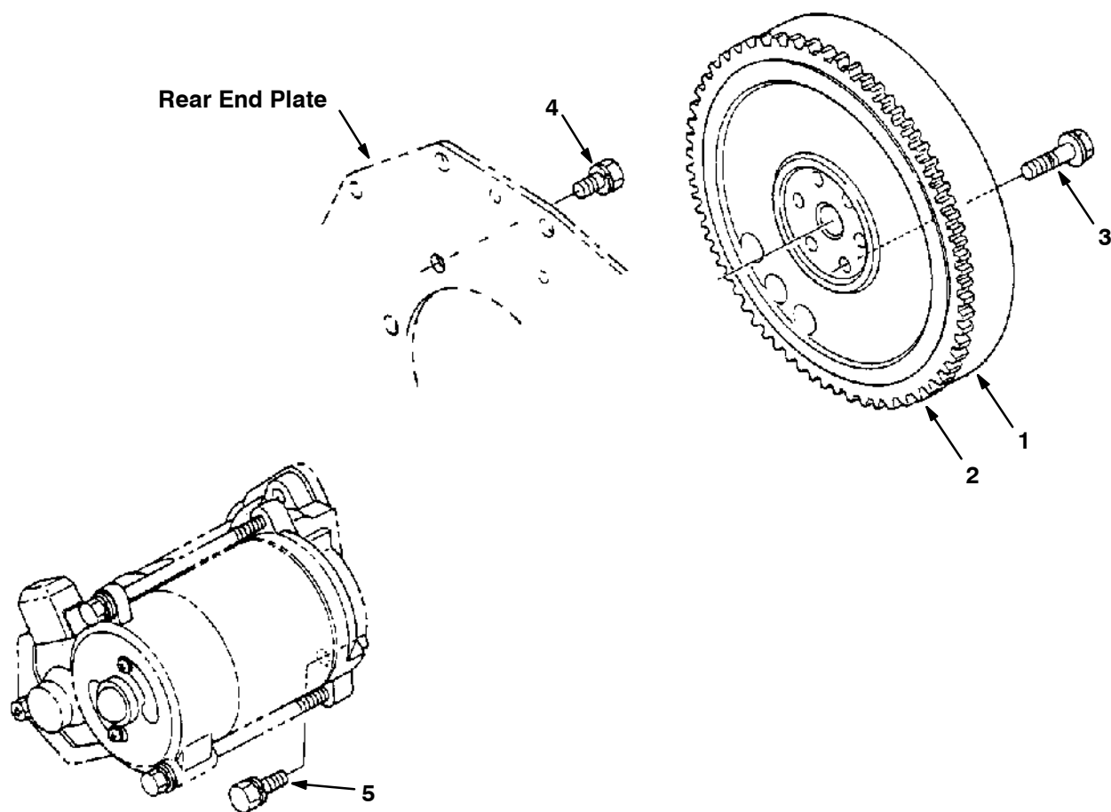
Fig. 12 - Flywheel Group
