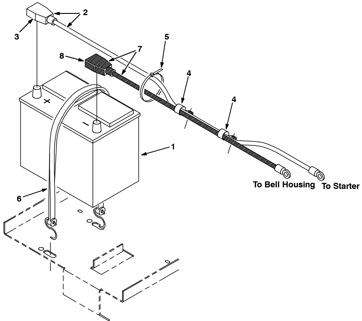
Fig. 24 - Battery Group
