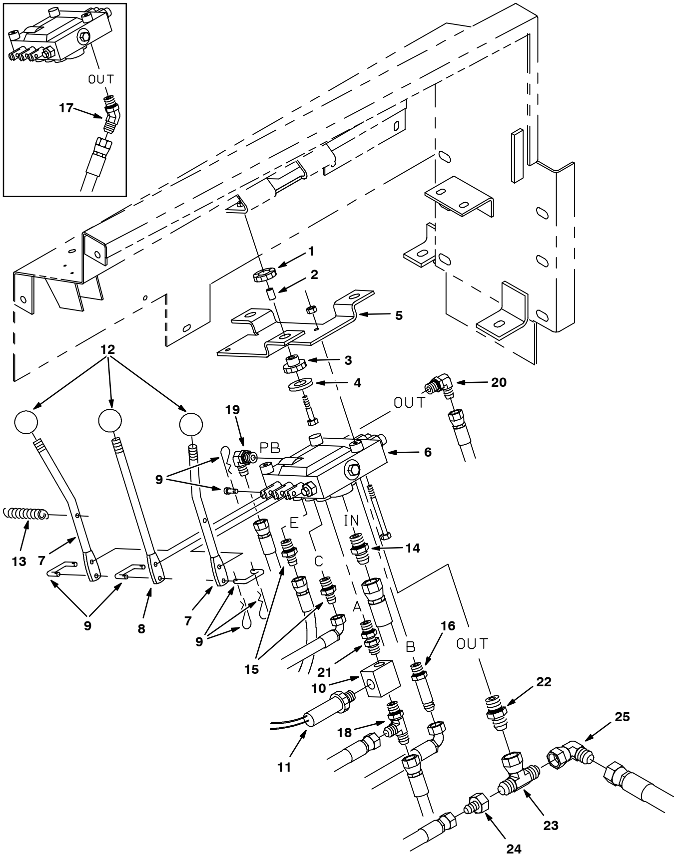
Fig. 47 - Hydraulic Valve Group
