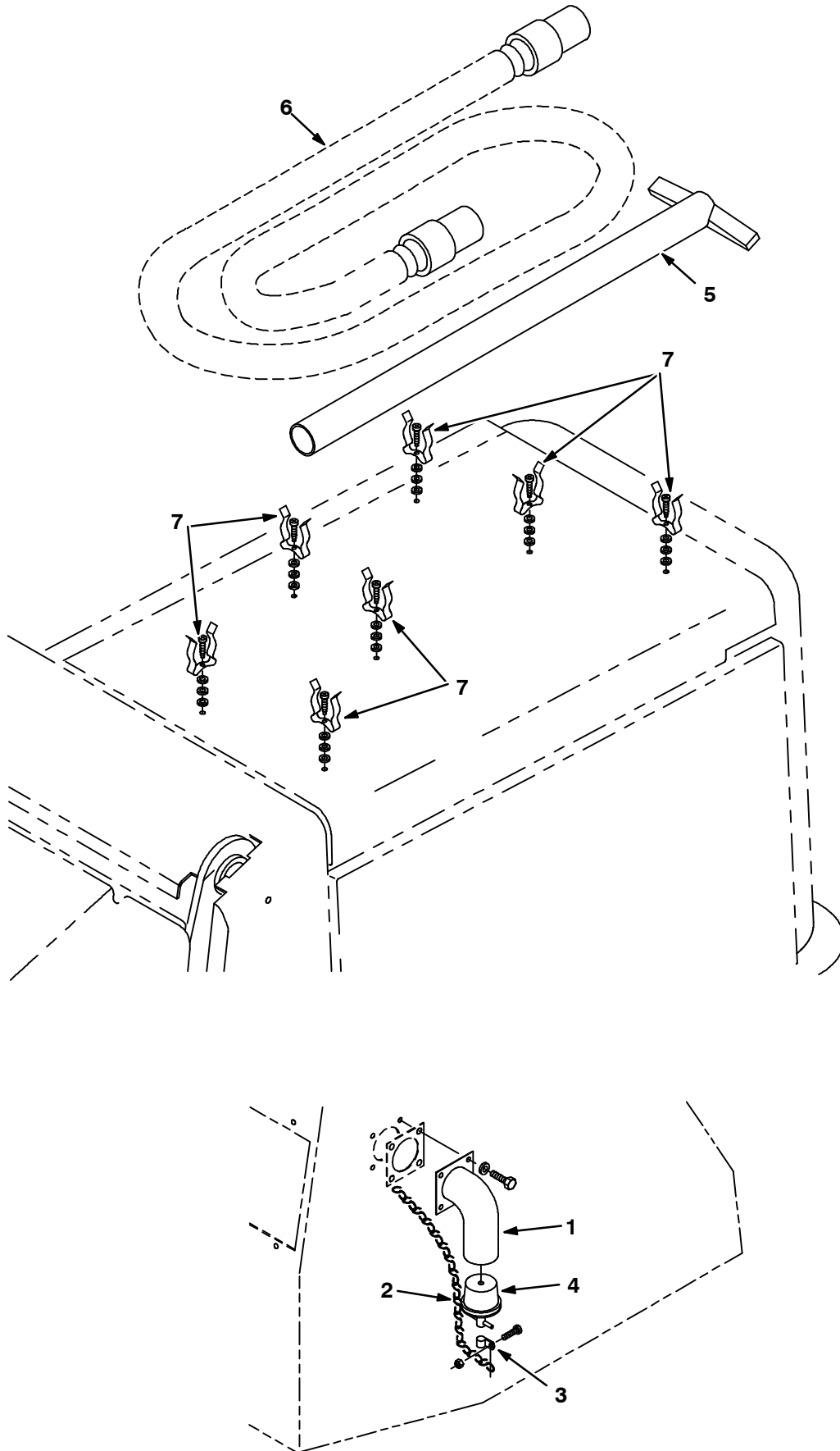
Fig. 18 - Vacuum Wand Kit
