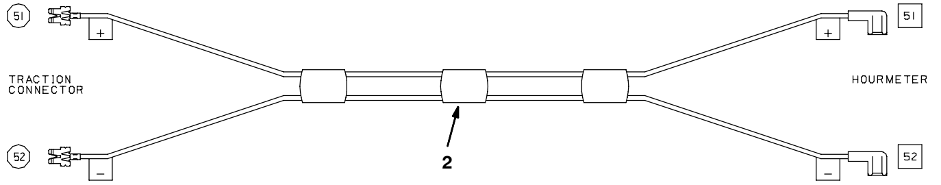
Fig. 32 - Wire Harnesses Group (10247590- )
