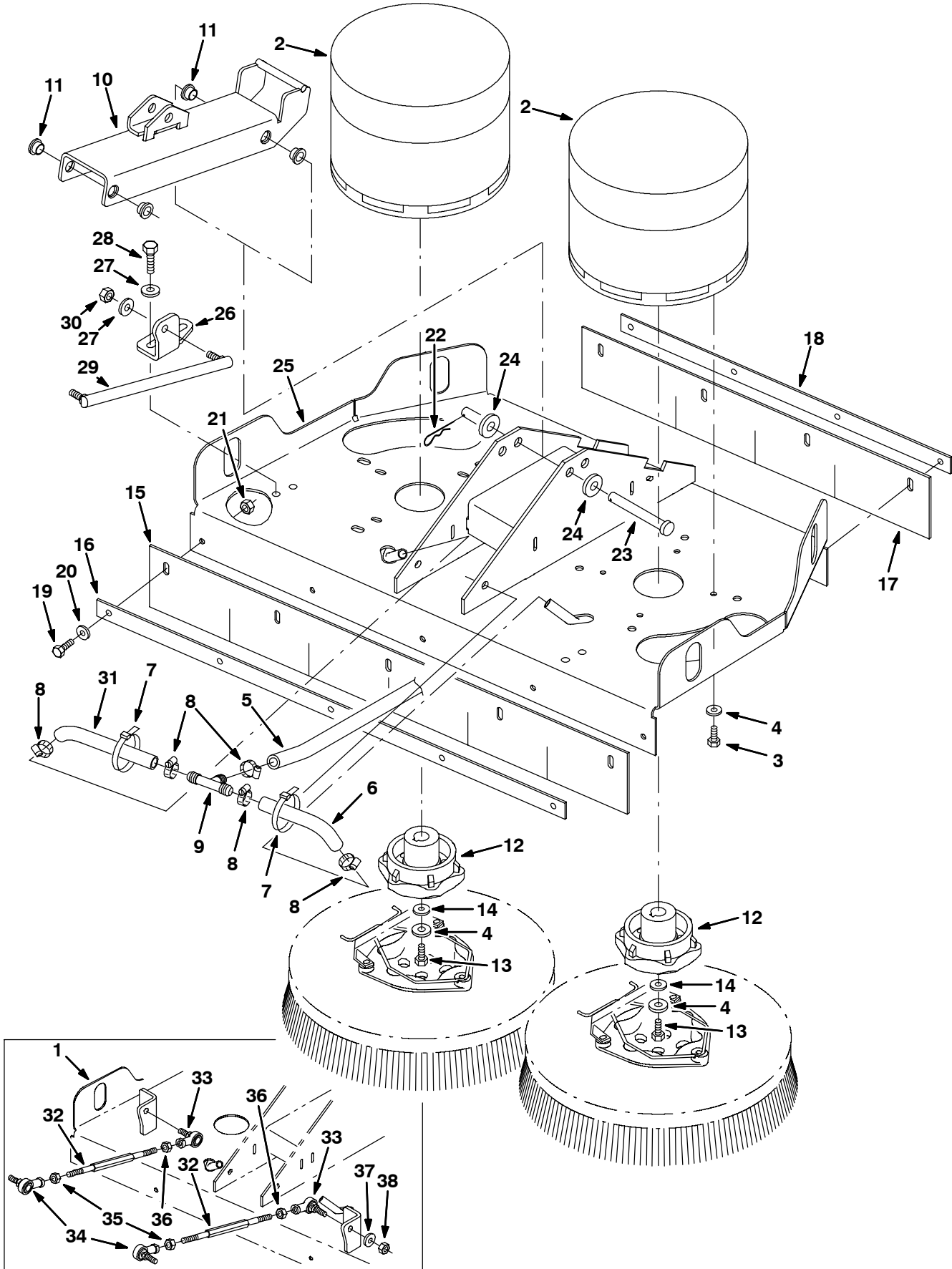
Fig. 12 - Heavy Duty Disk Scrub Head Drive Motor Group, 700 mm (28 in) (0000000-10214060)
