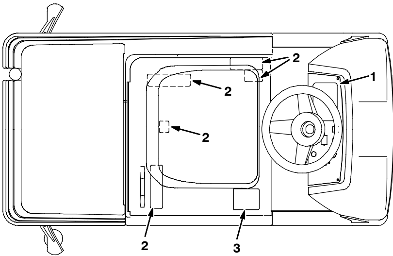
Fig. 33 - Label Group
