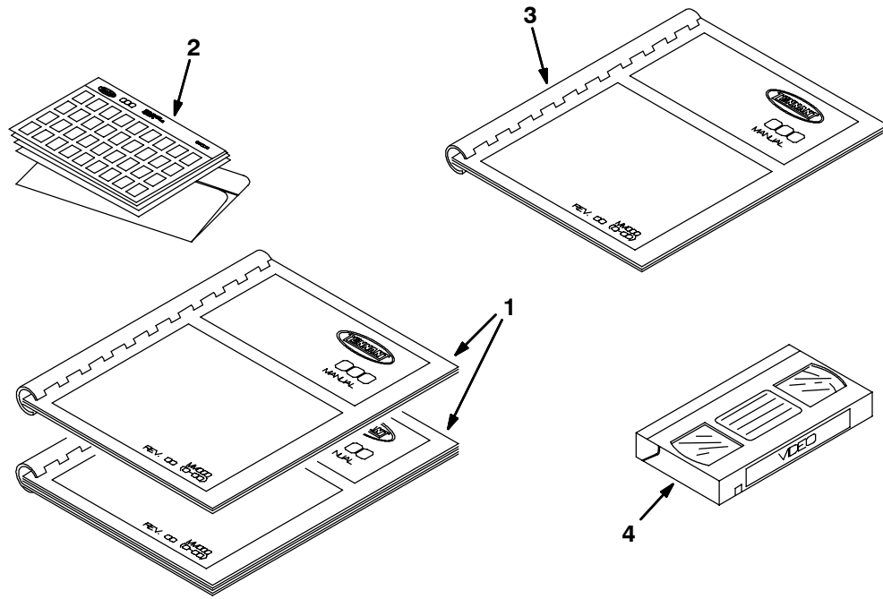
Fig. 35 - Documentation Group
