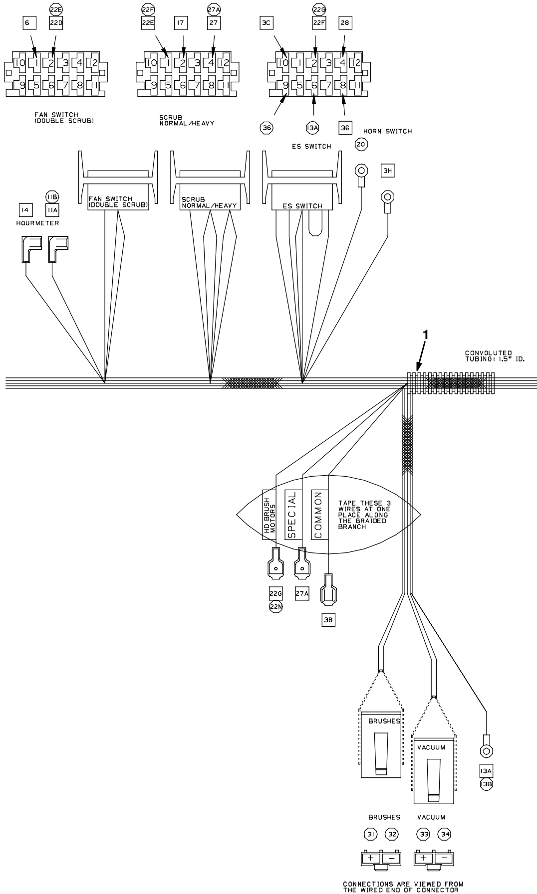
Fig. 30 - Wire Harnesses Group (0000000-10143032)
