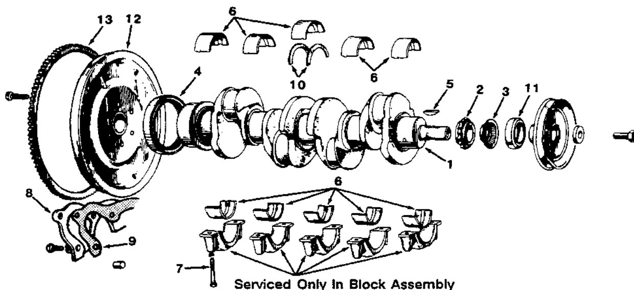
Fig. 2 - Crankshaft Group
