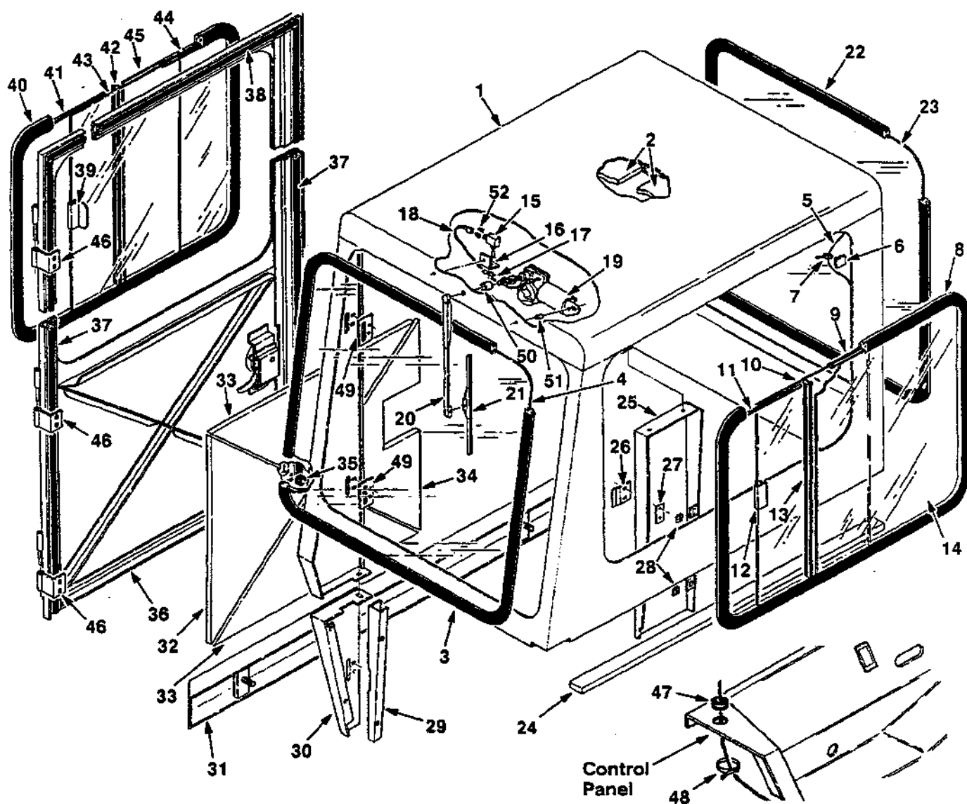
Fig. 1 - Cab Kit
