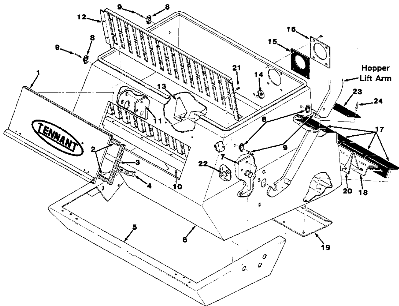
Fig. 6 - Hopper Group
