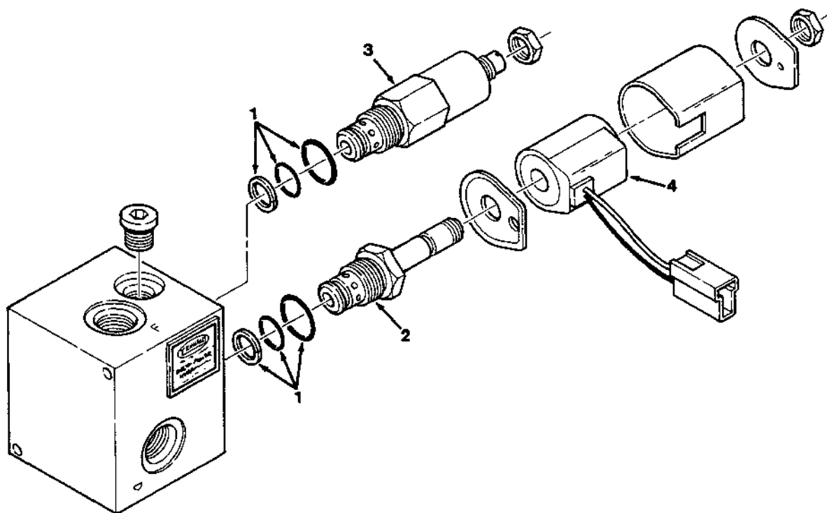
Fig. 13 - Hydraulic Solenoid Valve Breakdown
