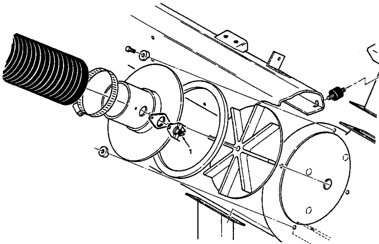
Fig. 46 - Thermostat Kit
