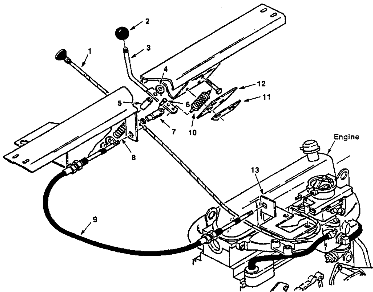
Fig. 33 - Throttle Linkage Group
