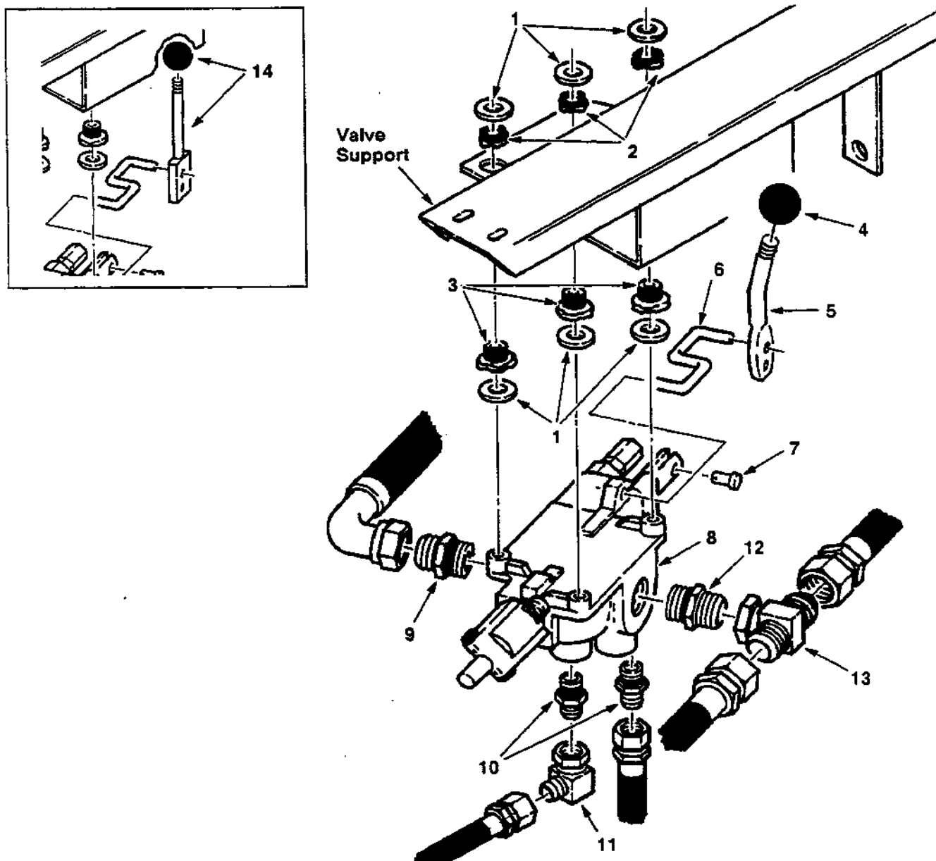
Fig. 24 - Hydraulic Control Valve Group
