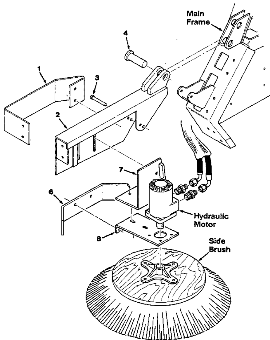
Fig. 8 - Side Brush Group, Multi-Level Dump
