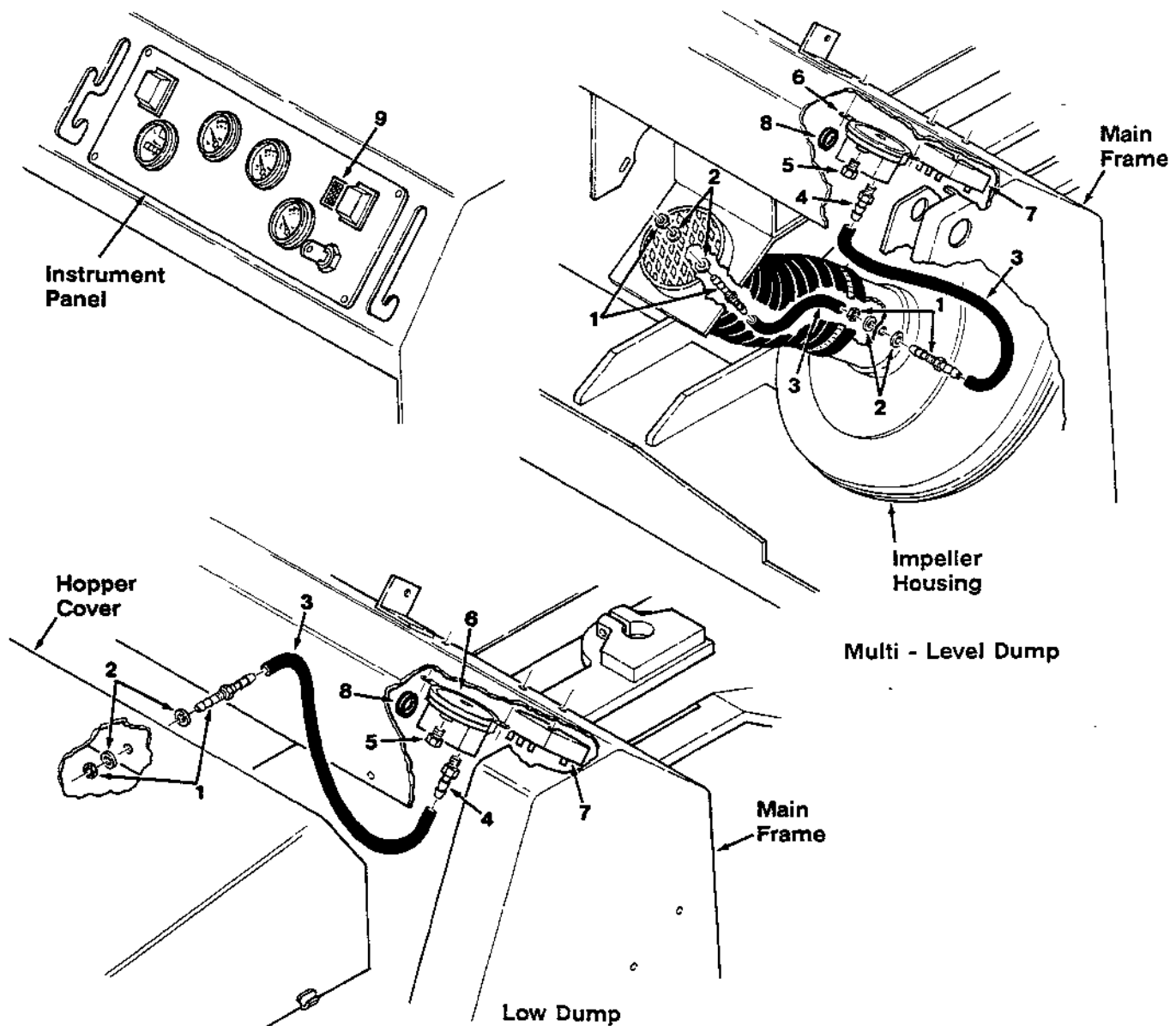
Fig. 28 - Clogged Filter Indicator Kit
