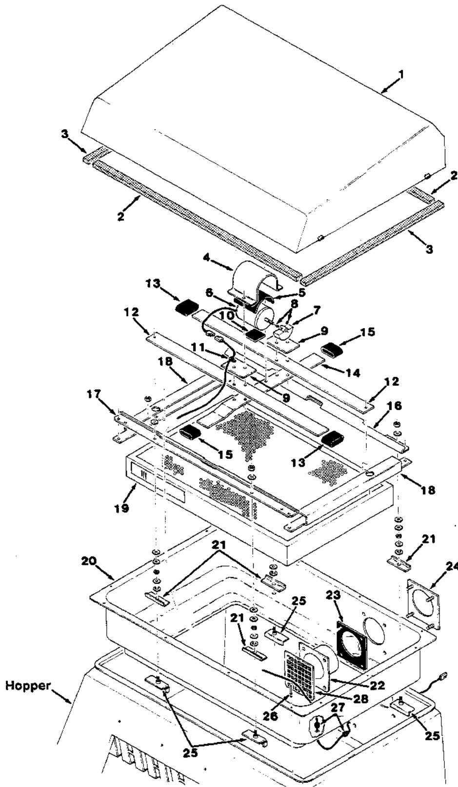
Fig. 7 - Hopper Cover and Filter Shaker Group
