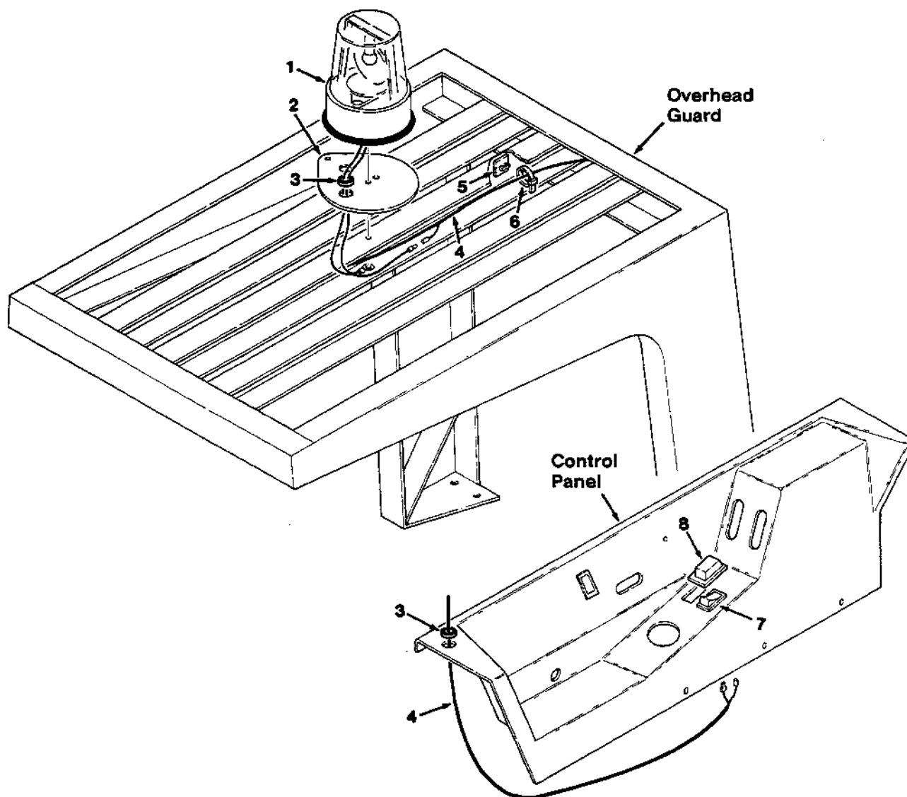
Fig. 10 - Revolving Light Kit, Overhead Guard
