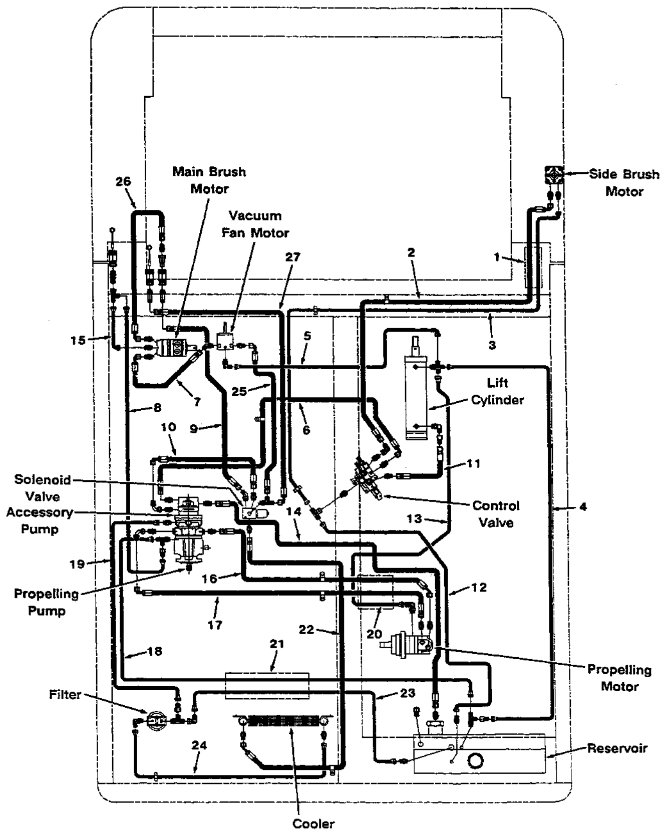
Fig. 21 - Hydraulic Hoses Group
