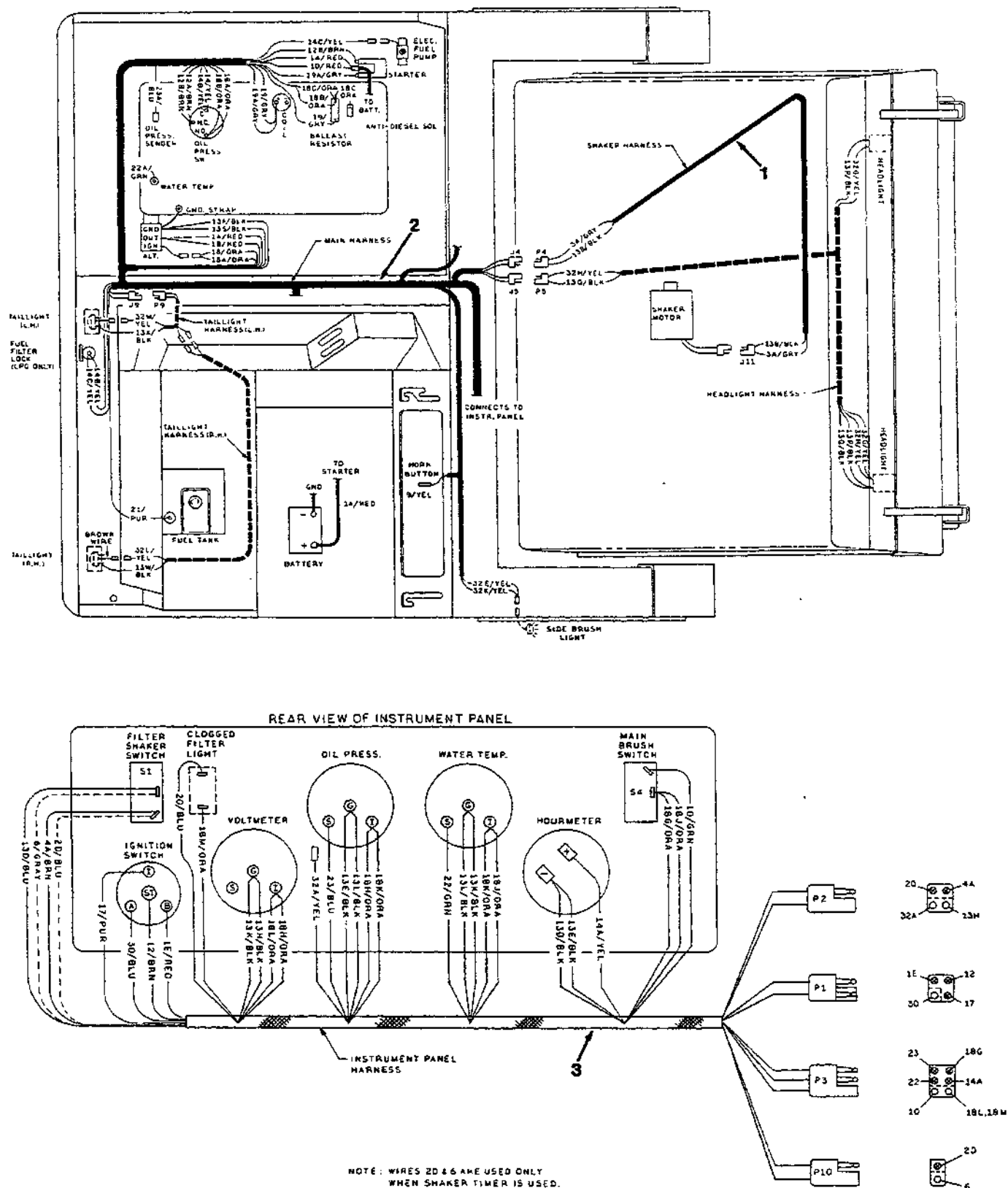
Fig. 19 - Wire Harnesses Group
