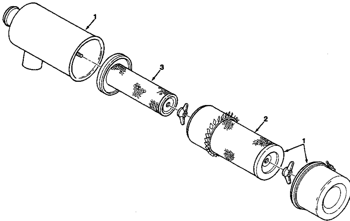
Fig. 27 - Air Cleaner Kit, Heavy Duty
