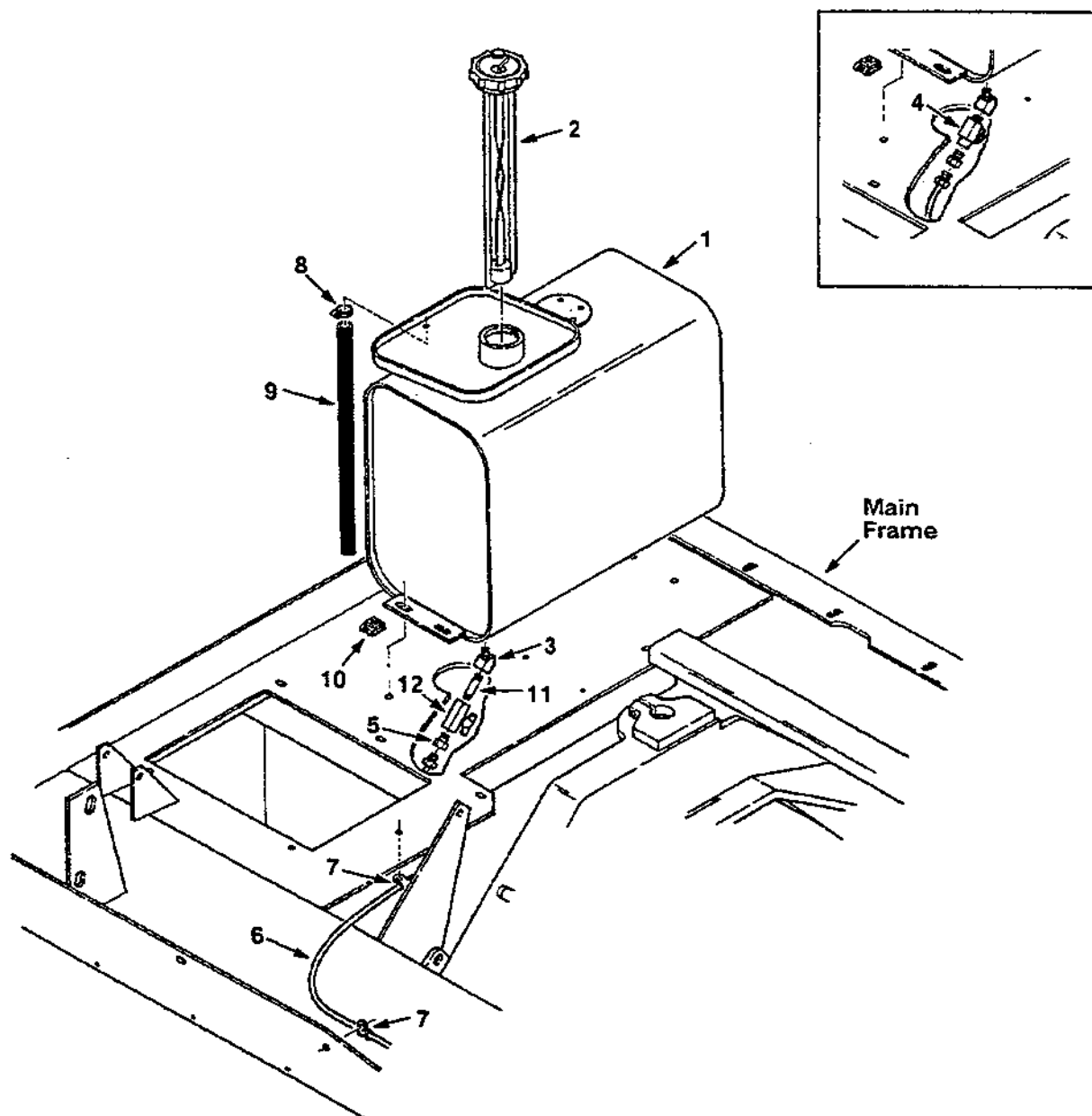
Fig. 35 - Fuel Tank Group
