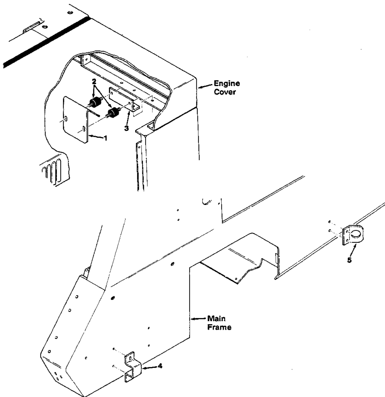
Fig. 43 - Hood Latch and Machine Tie-Down Kit
