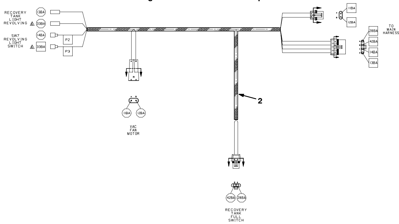
Fig. 27 - Wire Harnesses Group
