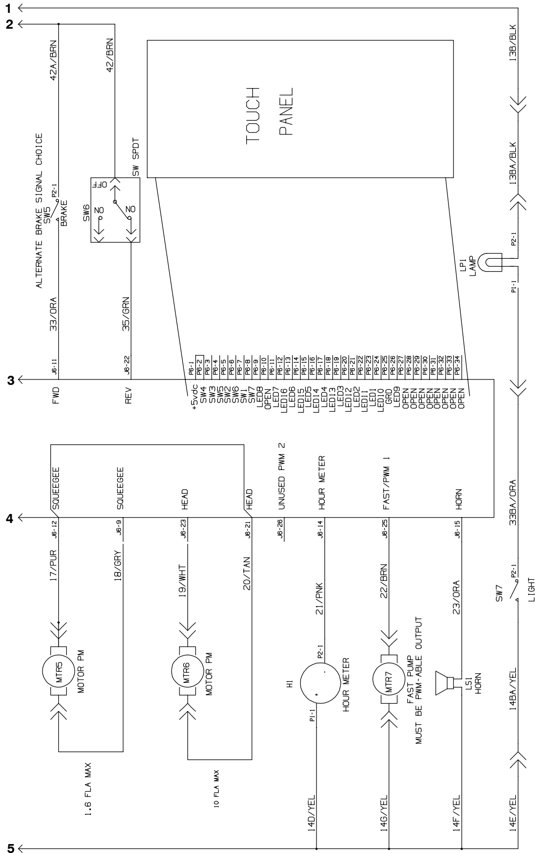
Fig. 26 - Electrical Schematic
