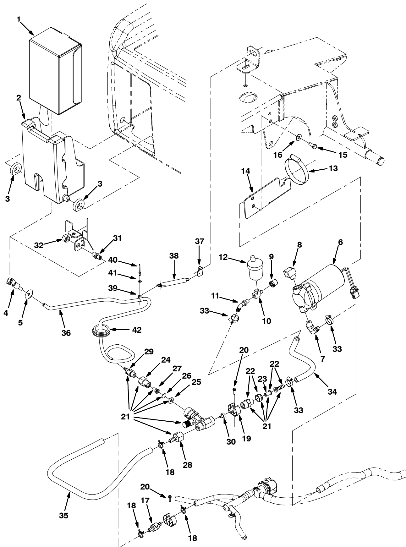
Fig. 1 - FaST Group
