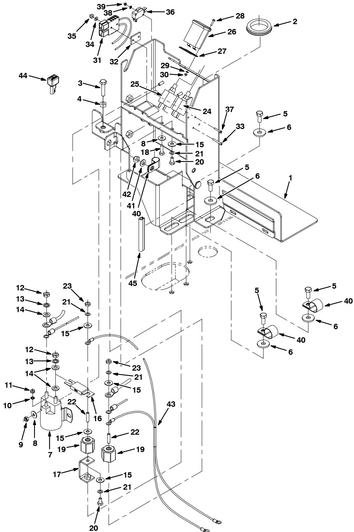
Fig. 25 - Electrical Group
