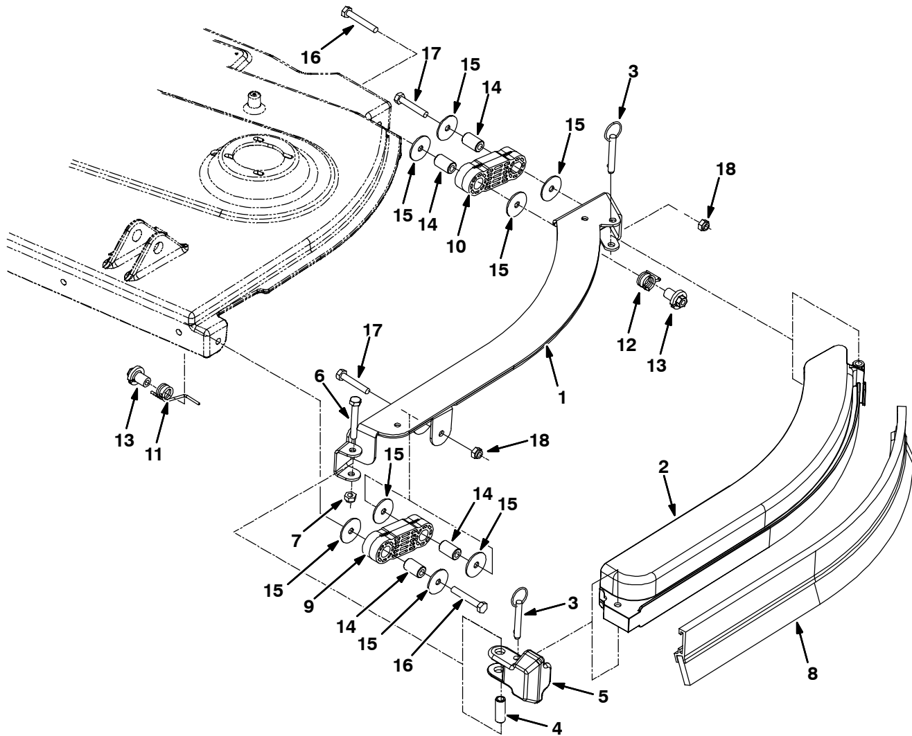
Fig. 14 - Side Squeegee Group, Left
