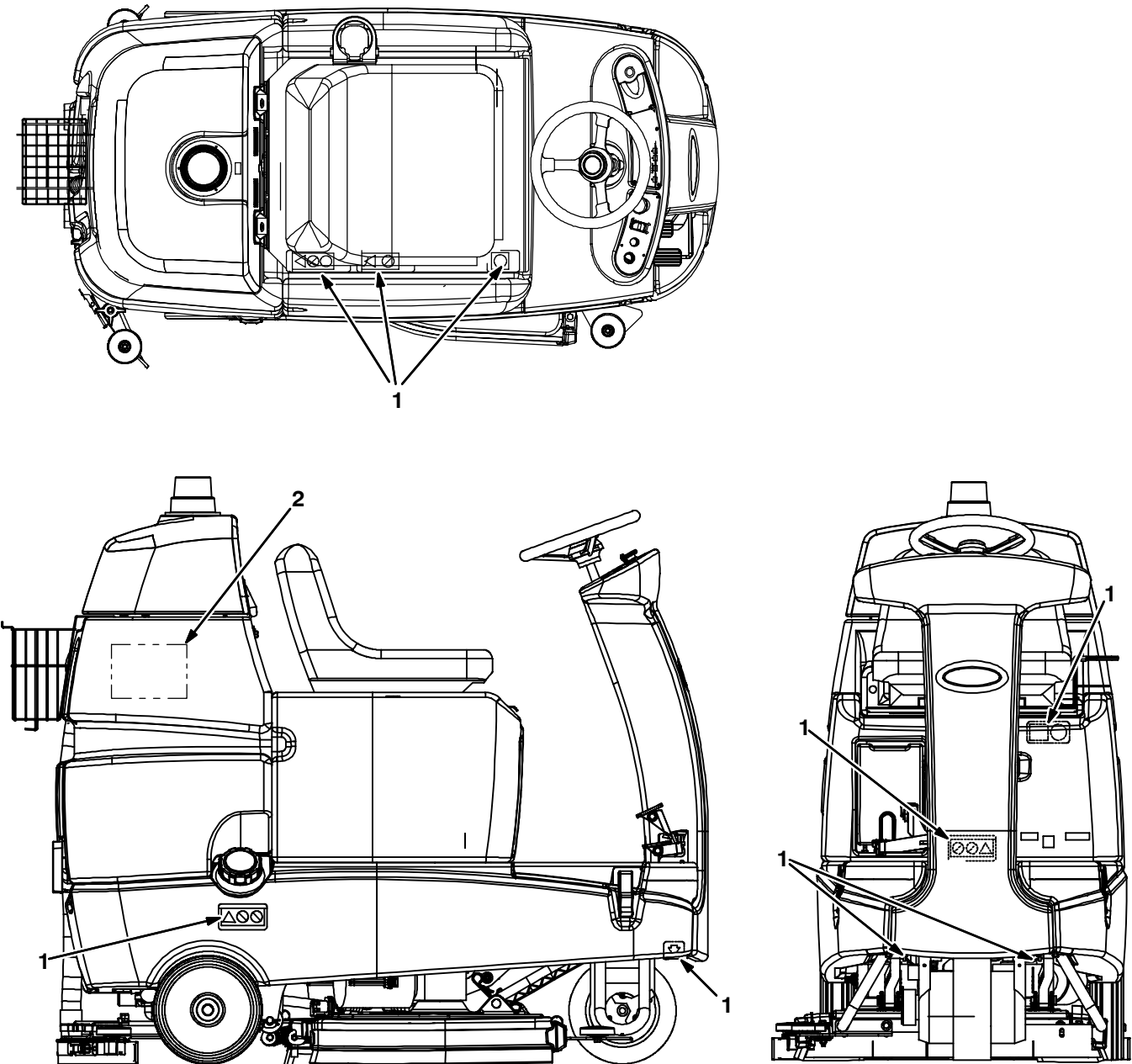
Fig. 28 - Label Group
