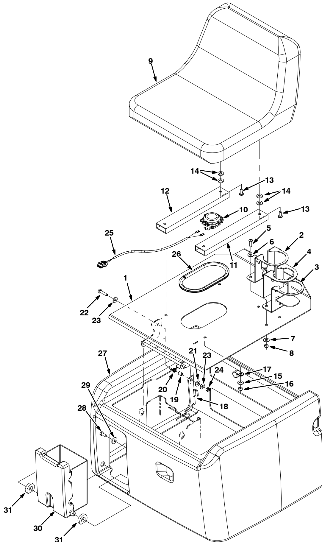
Fig. 5 - Seat Group
