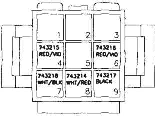
REAR VIEW OF CONNECTOR (740320)
